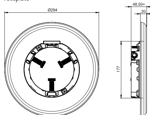
Faceplate
