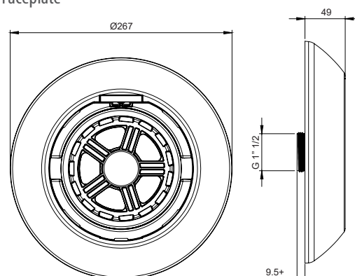
Faceplate
