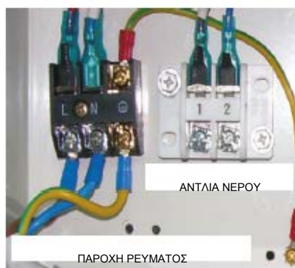
230V / 1ph / 50Hz
